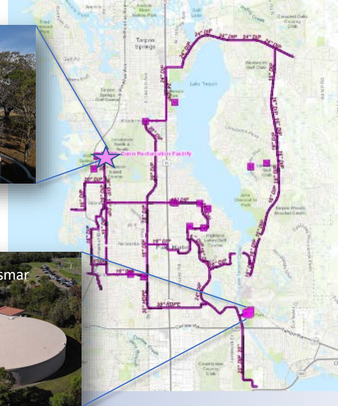
Dunn Reclaim Water Facility & Storage Pond
