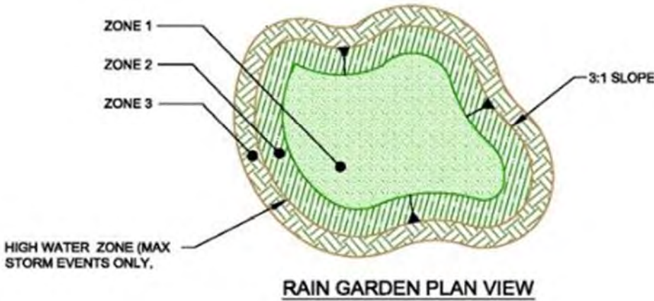
Figure 4.13.3: Rain garden plan view, provided by Applied Sciences, Inc.
