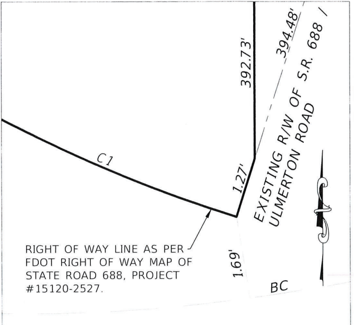
DETAIL #1 ~ SCALE 1" = 2'
