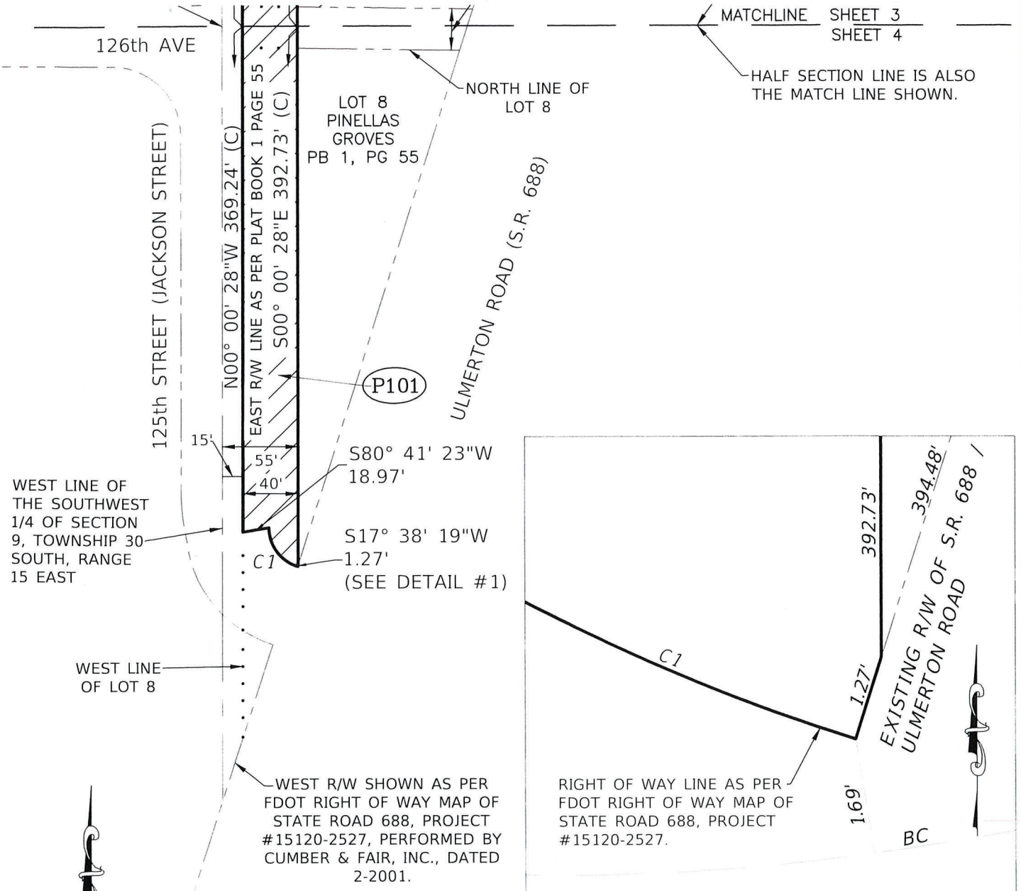
DETAIL #1 ~ SCALE 1" = 2'
