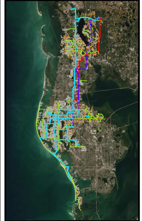
Water Distribution System + Water Booster Stations
