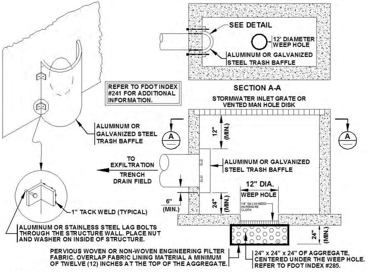
Figure 4.2.4. Detail for Exfiltration Trench Trash Baffle
