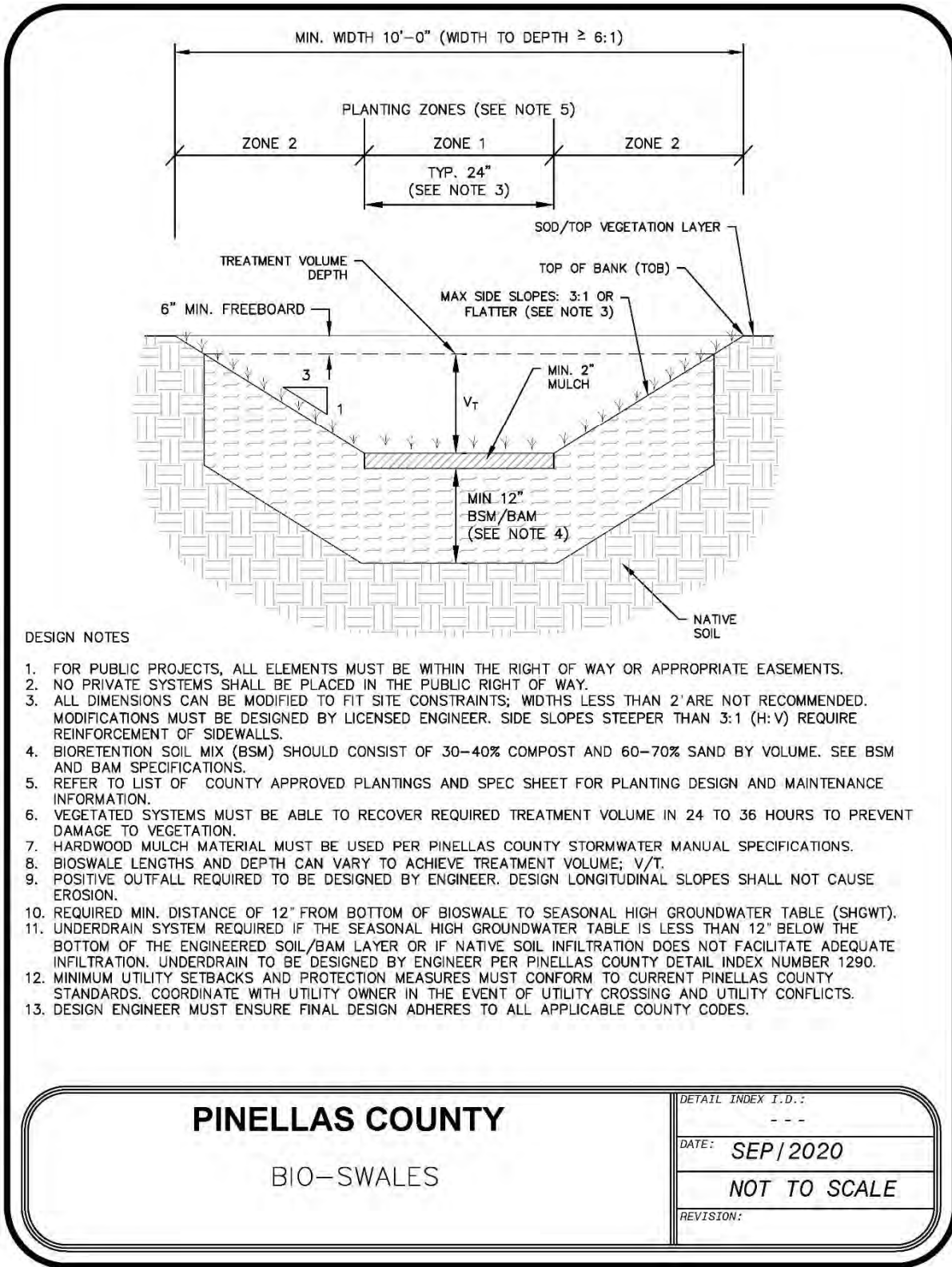
Figure 4.4.1. Pinellas County CAD template for bioswales
