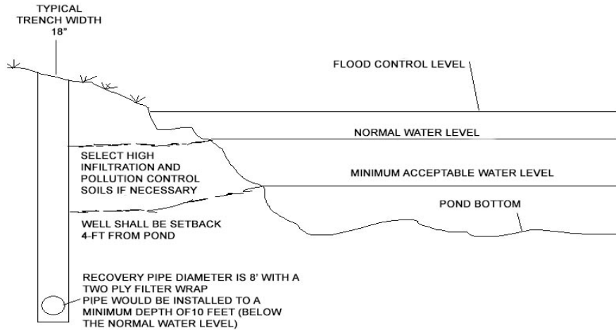
Figure 4.9.2. Schematic for a Typical Stormwater Harvesting Pond (from FDOT BD 521-03, Regional Stormwater Facilities, December 2007).
