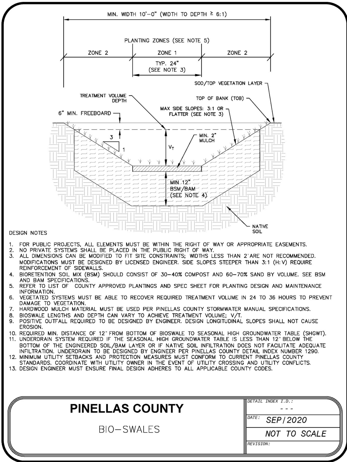
Figure 4.4.1. Pinellas County CAD template for bioswales
