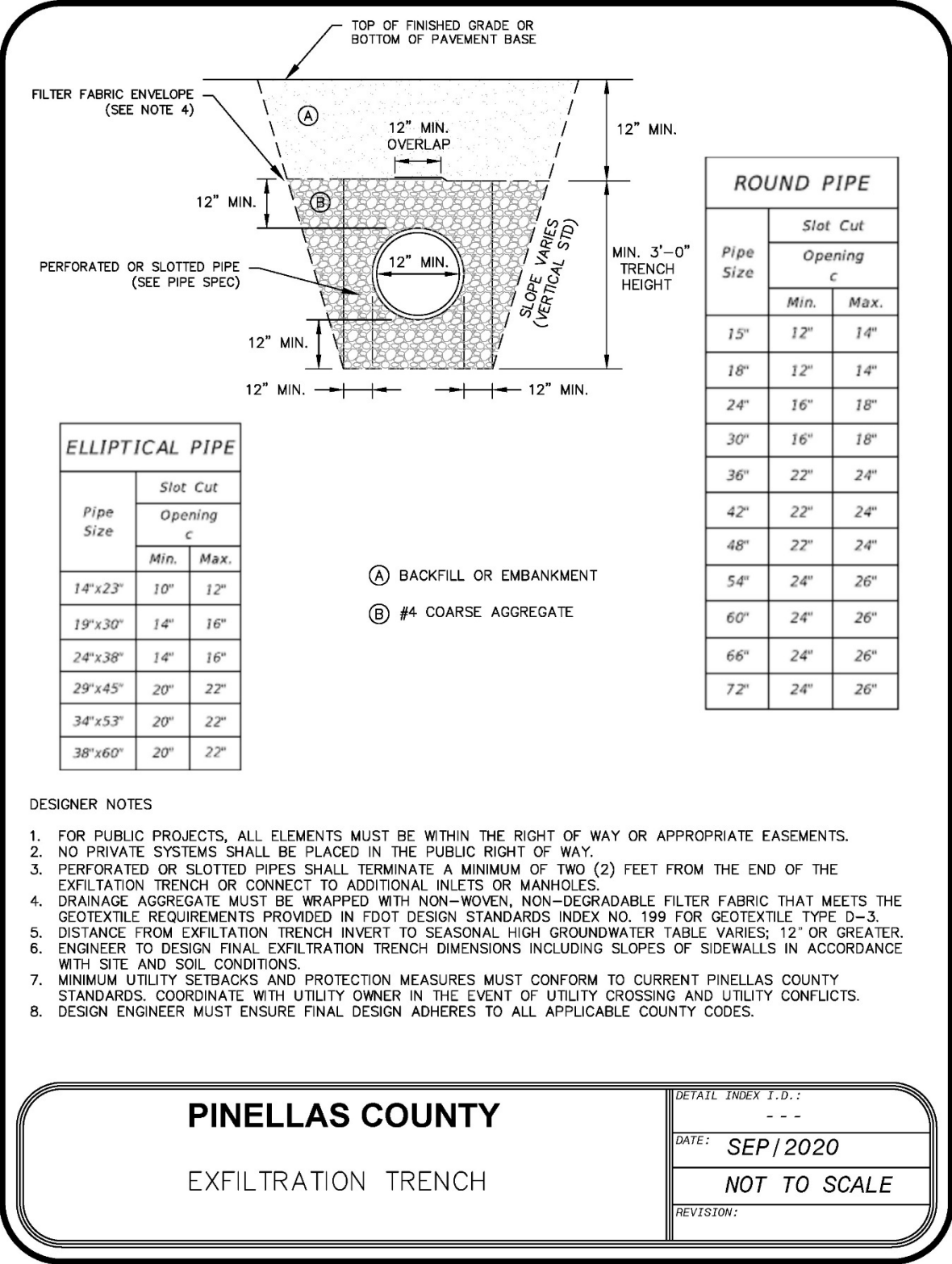
Figure 4.2.1: Pinellas County CAD template for exfiltration trenches
