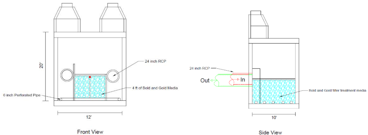
Figure 4.10.1. Front and Side Views of an Off-line Up-Flow Filter.
