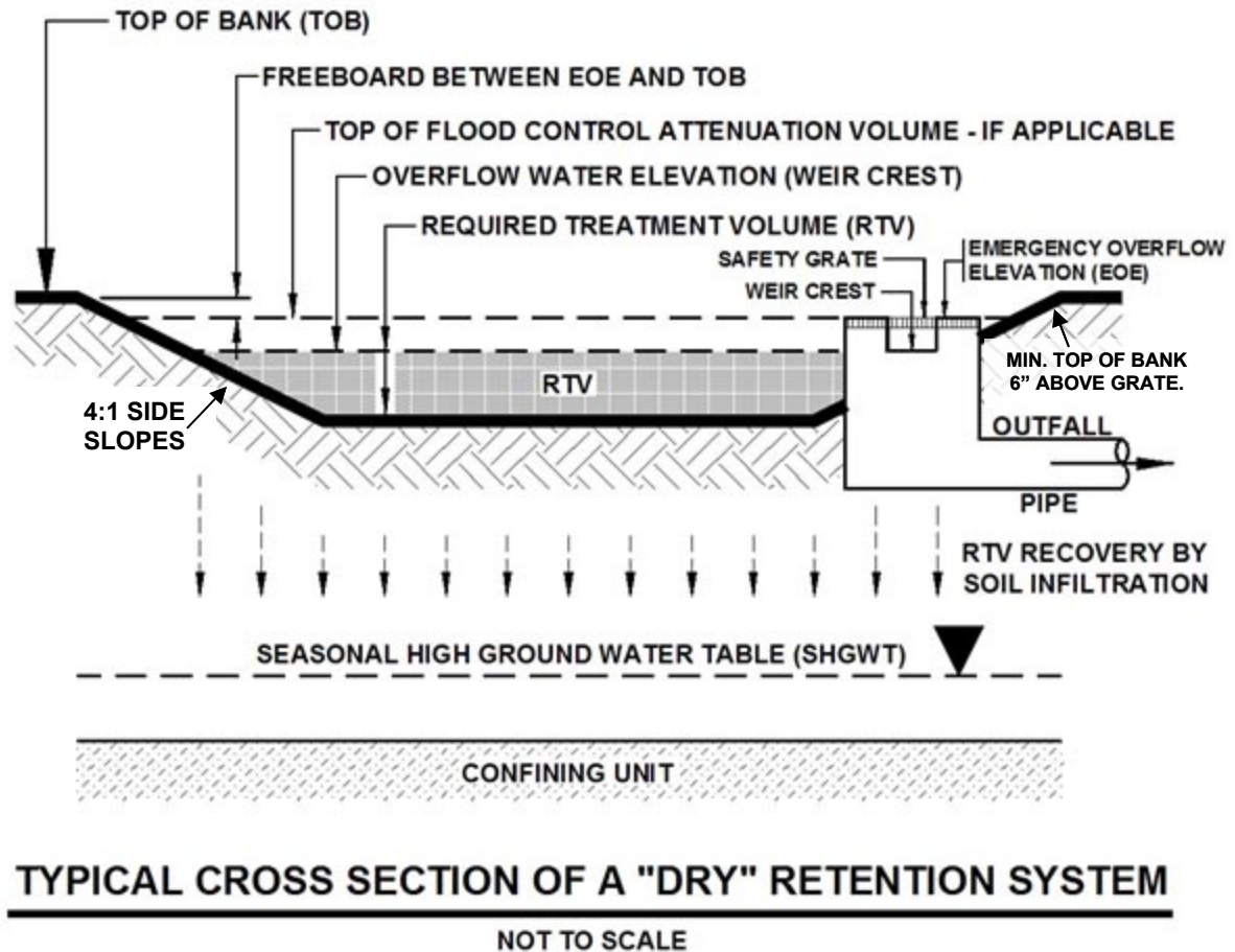
Figure 4.1.1. Typical Cross-section of "Dry" Retention Basin
