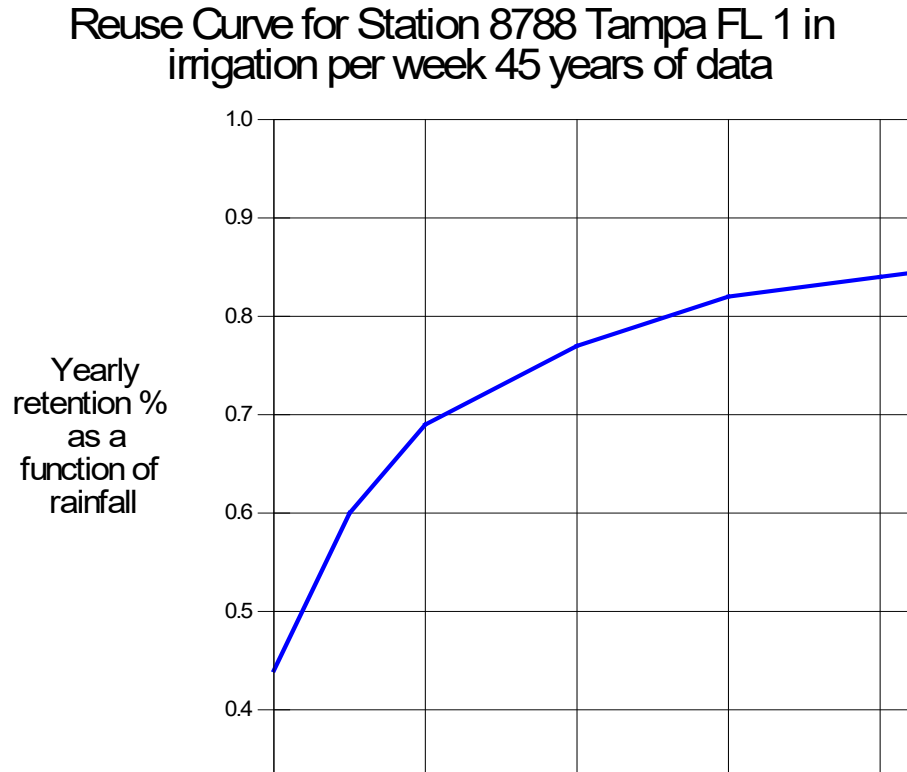
Figure 6.10.1. Greenroof Harvesting Design Curve for Tampa Florida Area Using 45 years of data.
