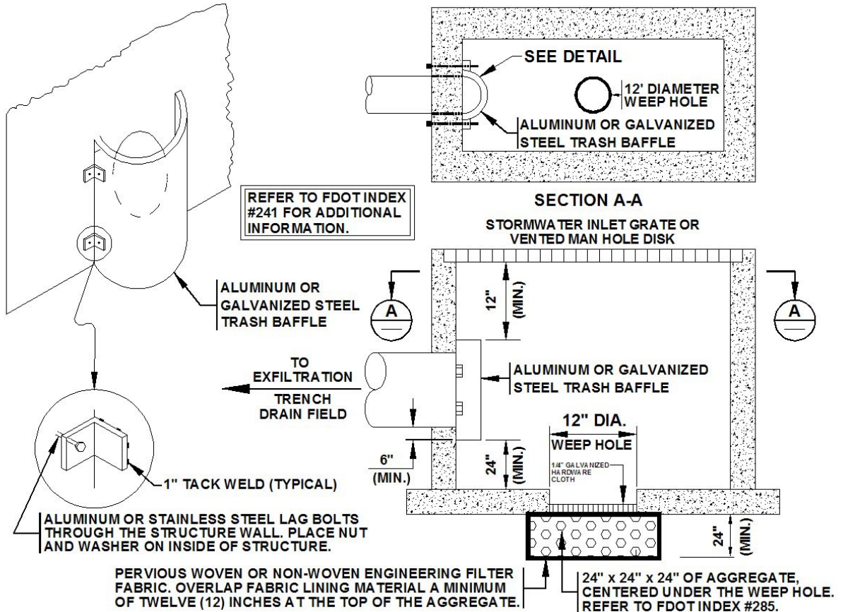
"GENERIC" DETAIL FOR AN EXFILTRATION TRENCH SEDIMENT / TRASH BAFFLE NOT TO SCALE
