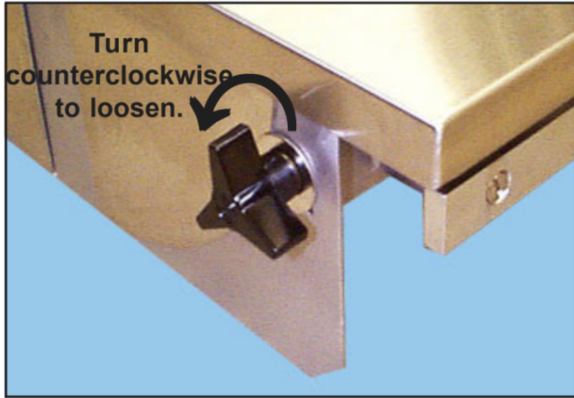
Figure 1. Top Panel Adjusting Knob (One of Four)
