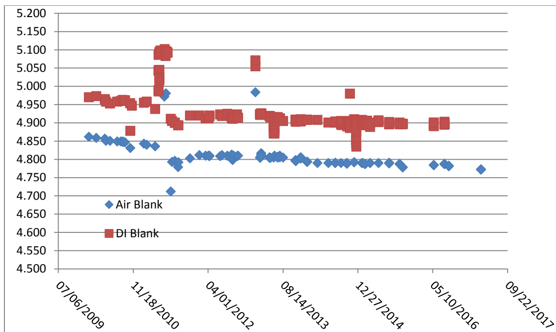
Figure 5: Transmissometer Air Blank and DI Blank Voltages.
