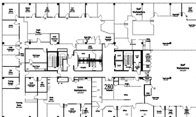
2 DEMO SECOND FLOOR PLAN SCALE: 3/32"=1'-0"
