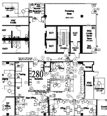
3 ENLARGE PARTIAL SECOND FLOOR PLAN SCALE: 1/8"=1'-0"
