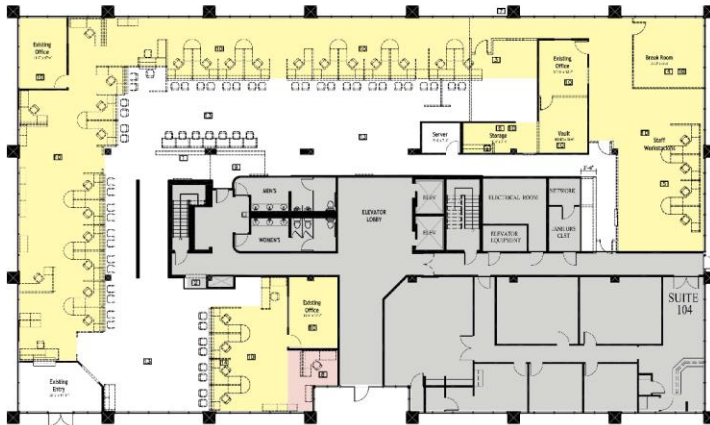
2 DEMO FIRST FLOOR PLAN SCALE: 3/32"=1'-0"
