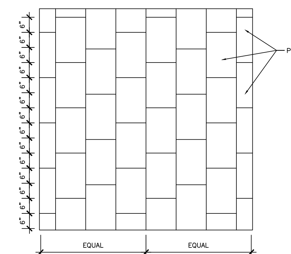
3. FLOORING PATTERN DETAIL 1/2" = 1'-0"
