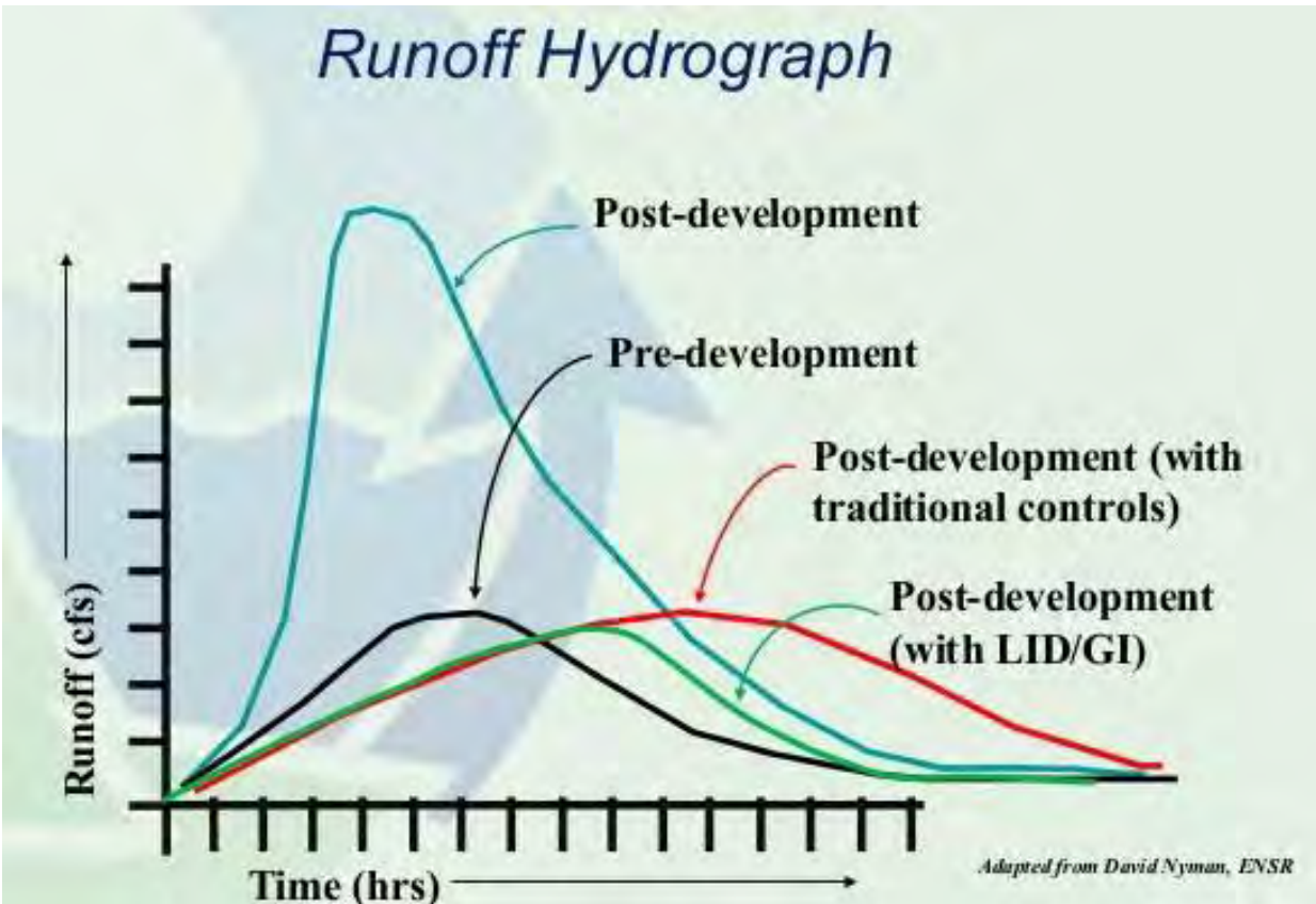
Figure 2.5.3. Hydrograph of LID stormwater infrastructure compared to traditional infrastructure management approaches. LID restores hydrograph behavior to better resemble pre-development flow patterns (Source: Horsley Witten Group, Inc.).
