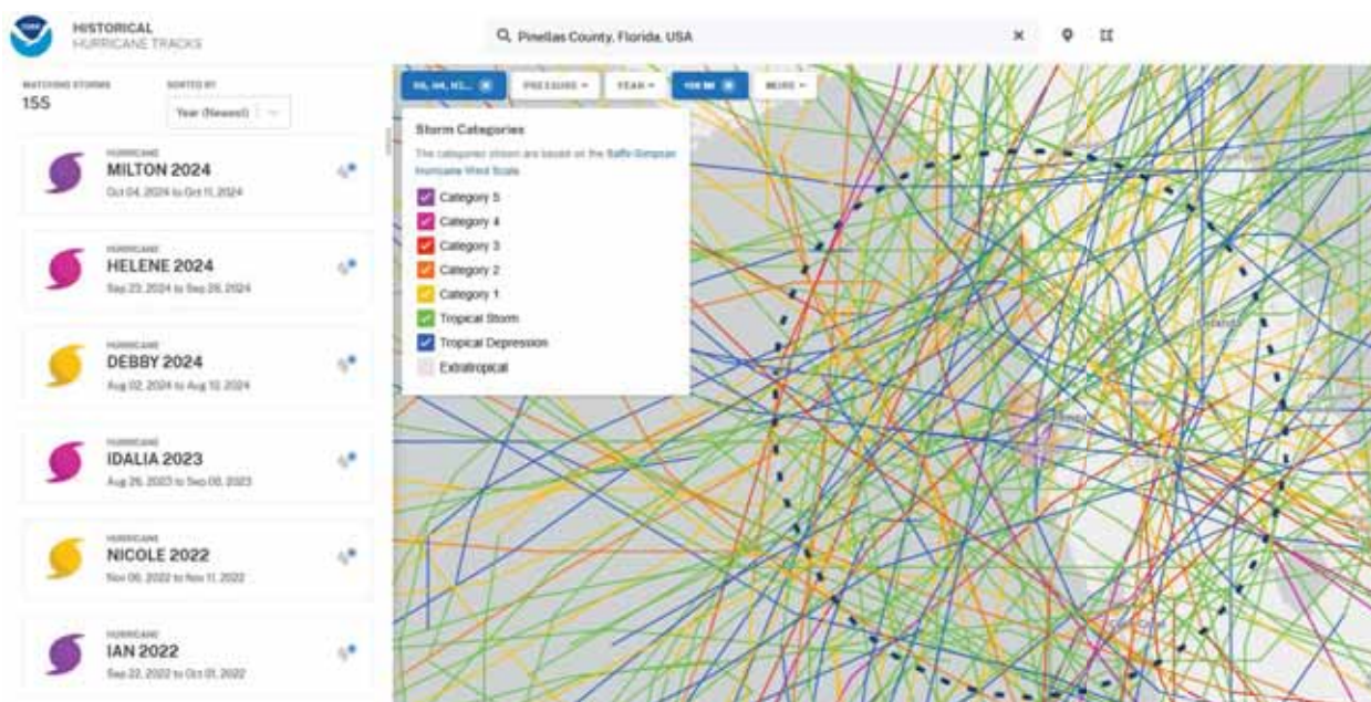
Figure 7: Tropical events within 100 Miles of Pinellas County
