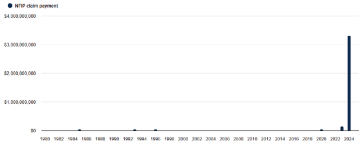
Figure 2: NFIP claim payments in Pinellas County, Florida through 2025 (floodsmart.gov/historical-nfip-claims-information-and-trends)
