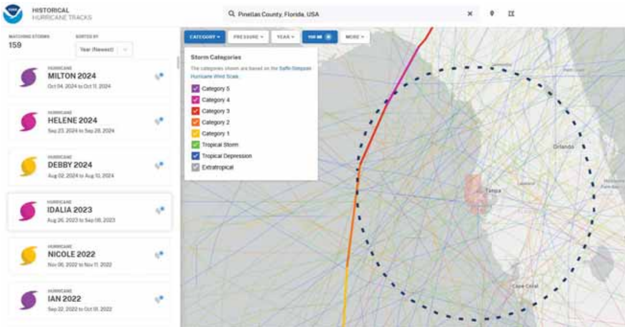
Figure 10: Hurricane Idalia Track 2023
