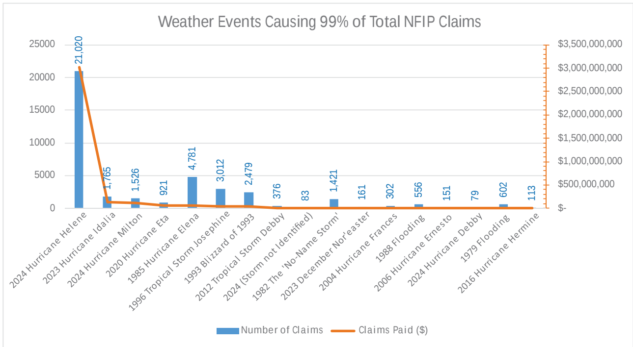
Figure 13: Weather Events Causing 99% of Total NFIP Claims
