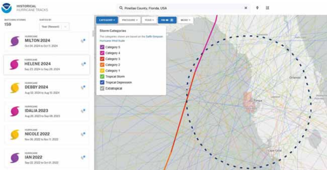
Figure 11: Hurricane Helene Track 2024
