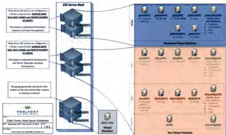
Figure 8 - Example Virtual (VM) Server Diagram Supporting a 4-Tier AMS Solution Deployment
