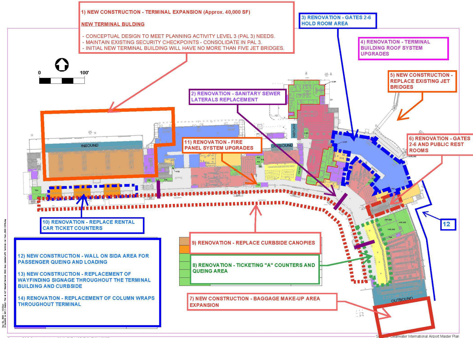
FIGURE 2.2-2 PASSENGER TERMINAL - FIRST FLOOR PLAN
